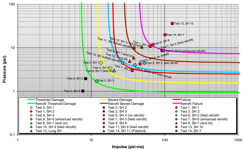
Figure A4.39. Standard and Retrofitted SEA Hut Response
