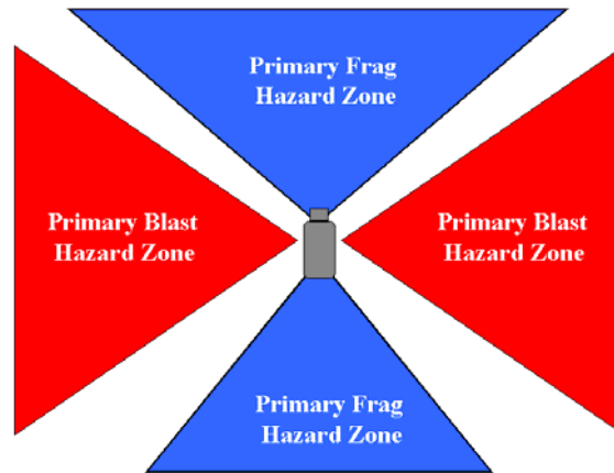
Figure 3.20. Blast and Fragment Hazard Zones
