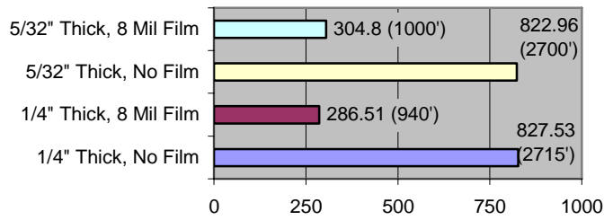
1219.20 mm x 1524 mm (48" x 60") Window Hazard Distances in Meters (ft) - No Blast Wall
